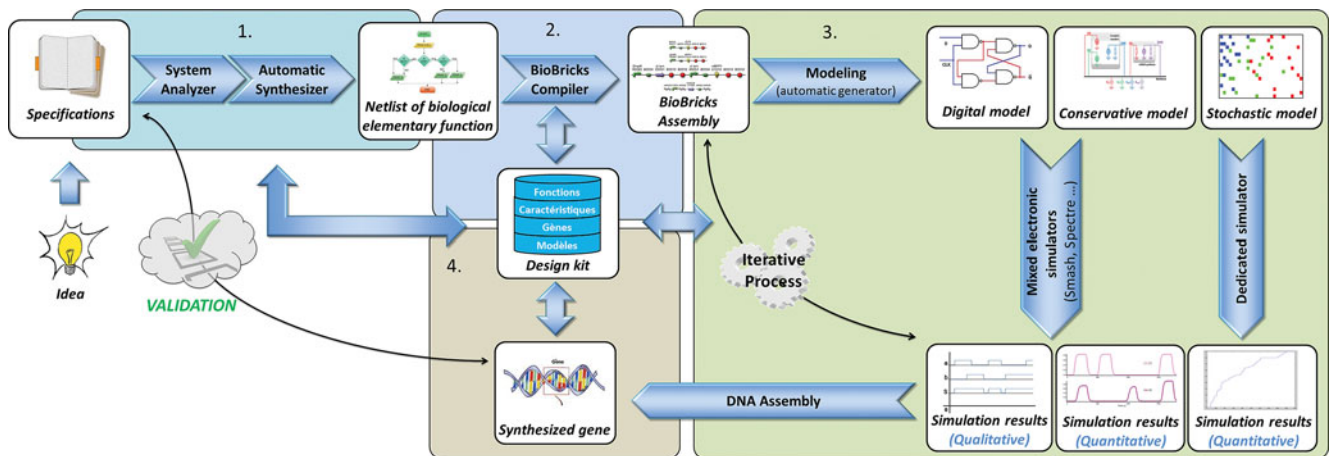
Scheme of the global project of a GDA tool for synthetic biology, based on electronic languages. As shown in “Modeling Biology With HDL Languages: A First Step Toward a Genetic Design Automation Tool Inspired From Microelectronics,” by Gendrault et al. , p. 1233.
